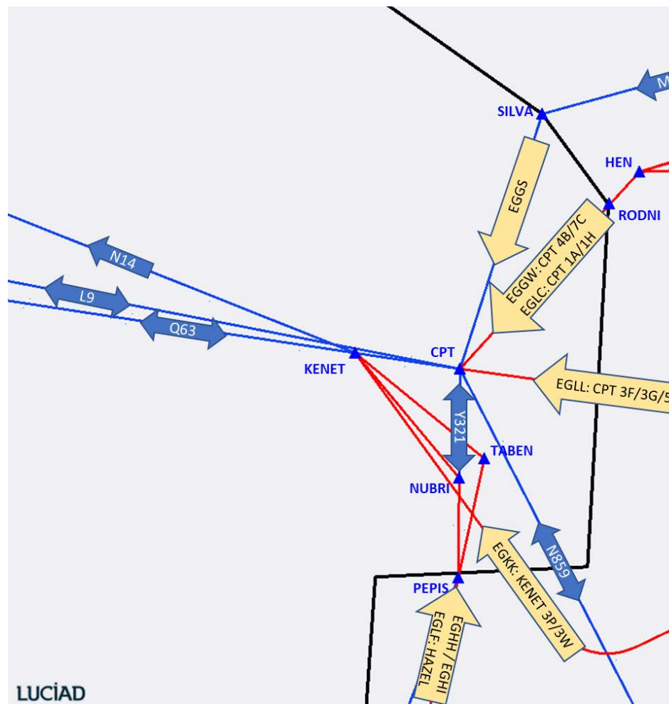
Figure 51 LTMA Baseline (Extant) Departure Connectivity via CPT
