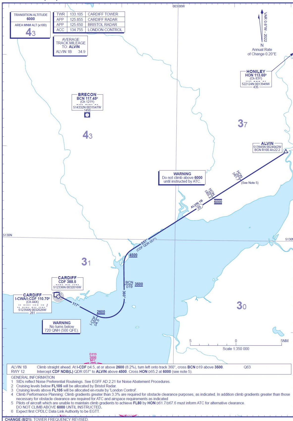
Figure 28 Extant Cardiff ALVIN 1B SID
