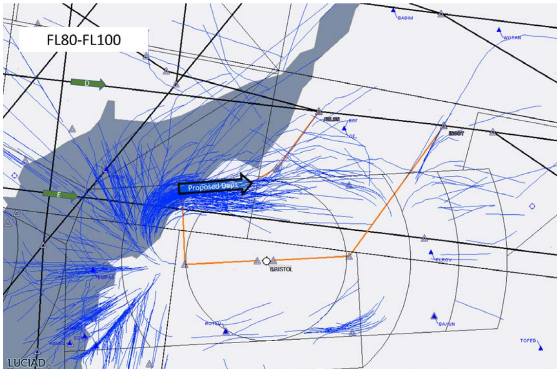
Figure 21 Bristol departures FL80-100, and proposed truncated SIDs
