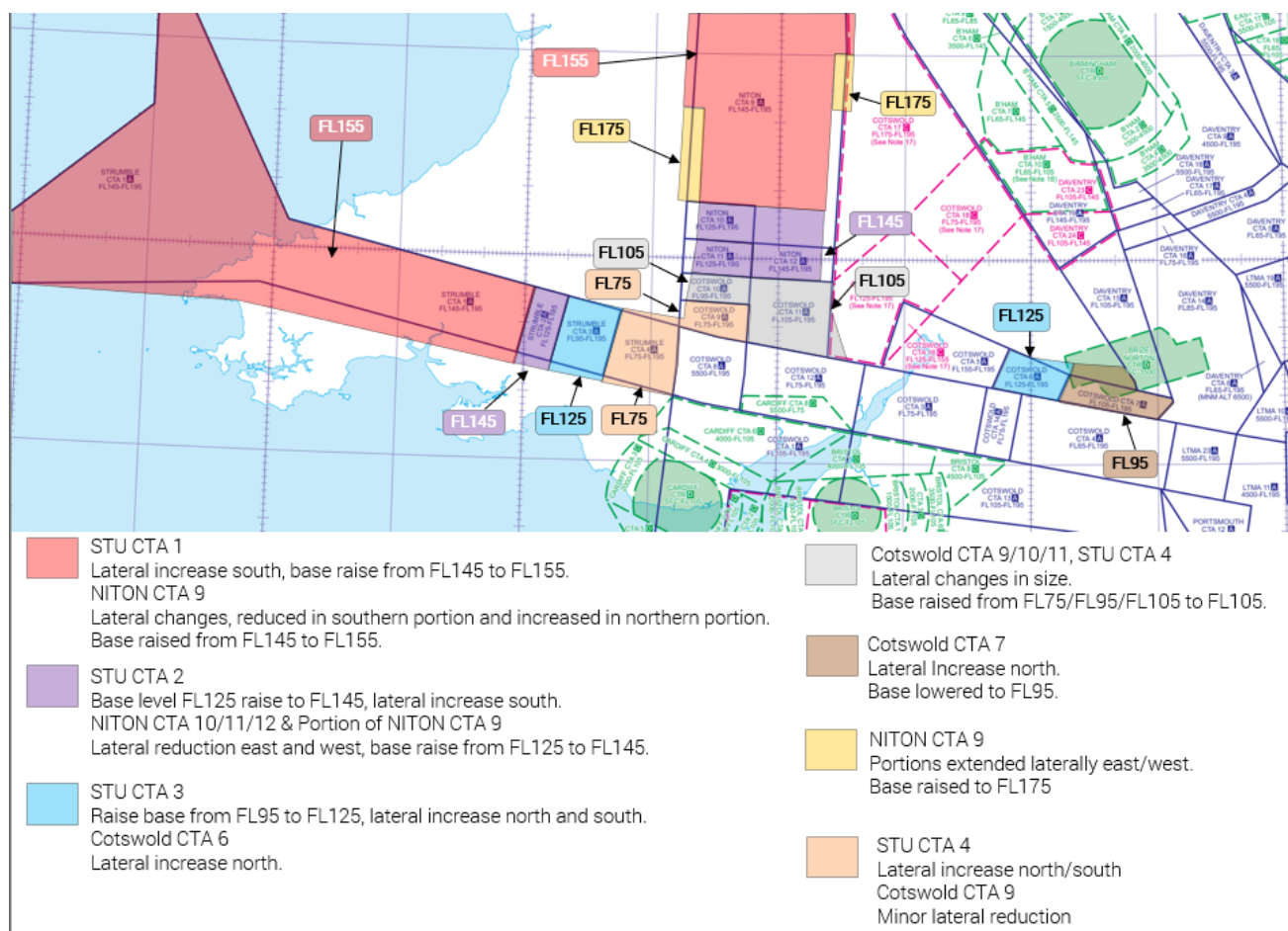
Figure 9 CAS changes in STU, NITON, Cotswold CTAs
