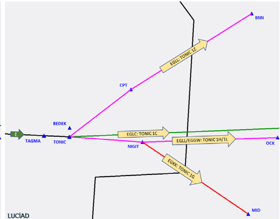
Figure 46 LTMA Proposed arrival routes: TONIC STARs (via Route E)
