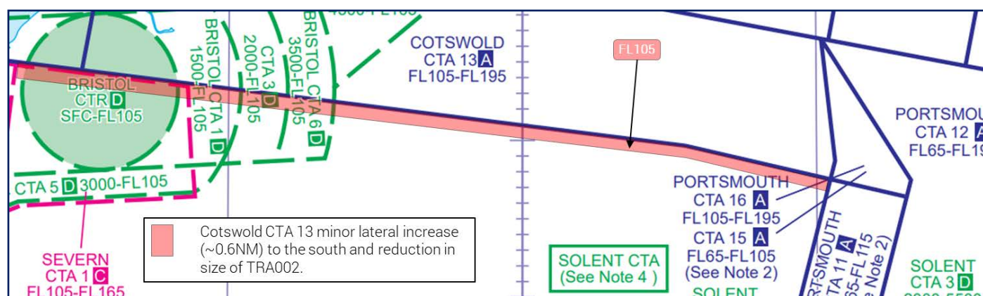
Figure 10 CAS changes: lateral increase in Cotswold CTA and reduction of TRA002
