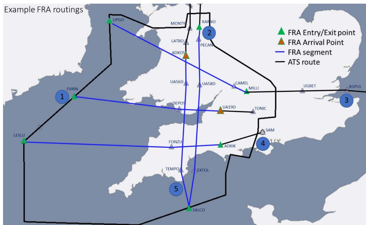
Figure 17 Example FRA routings
