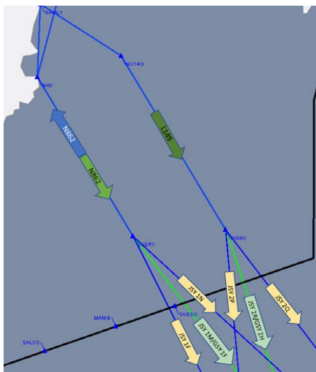
Figure 40 Channel Islands Group Extant Arrival connectivity
