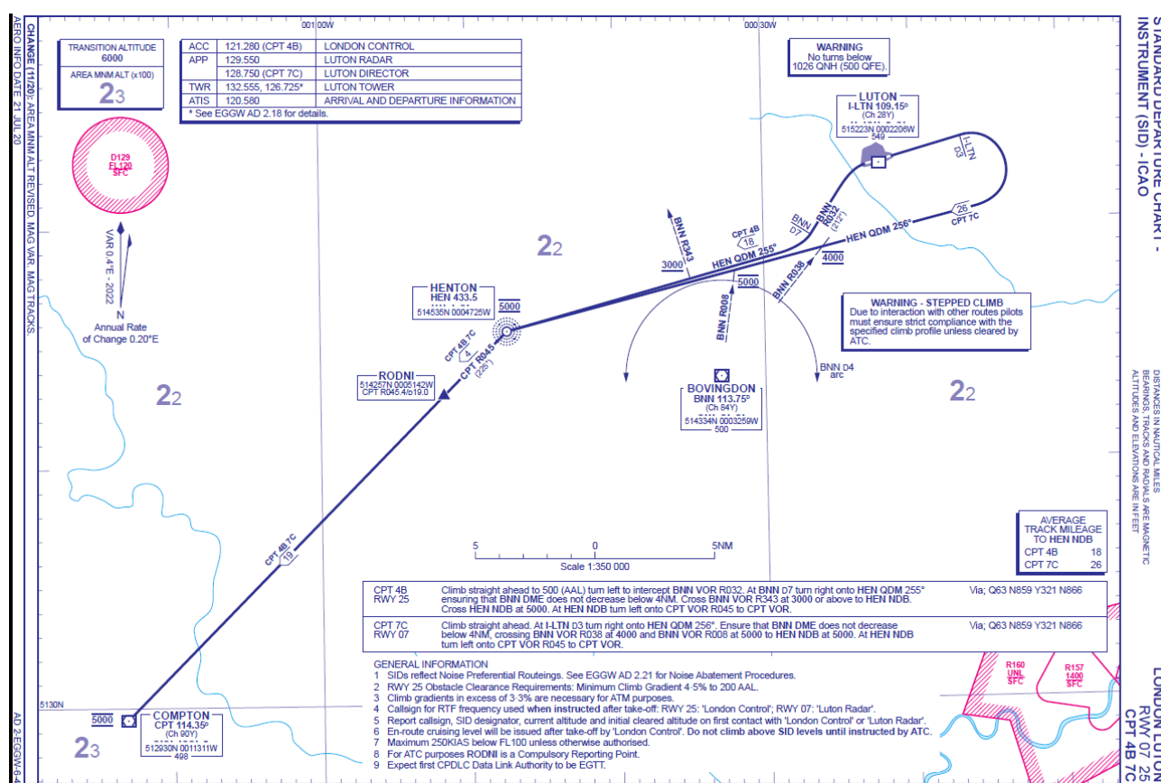
Figure 49 Extant Luton CPT 4B & 7C SIDs
