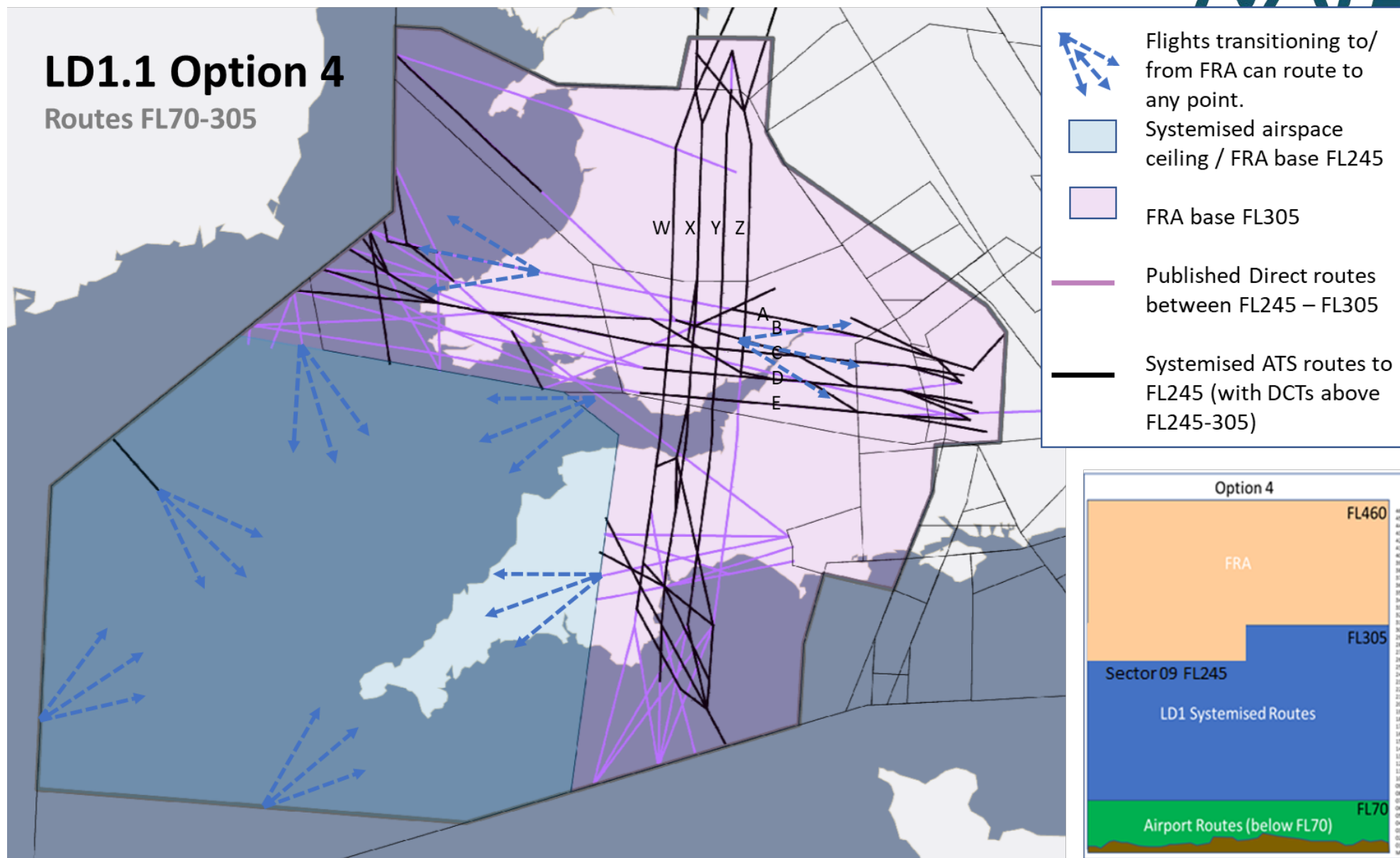
Figure 7 Option 4: Change to systemised routes FL70-305 with indicative FRA transitions
