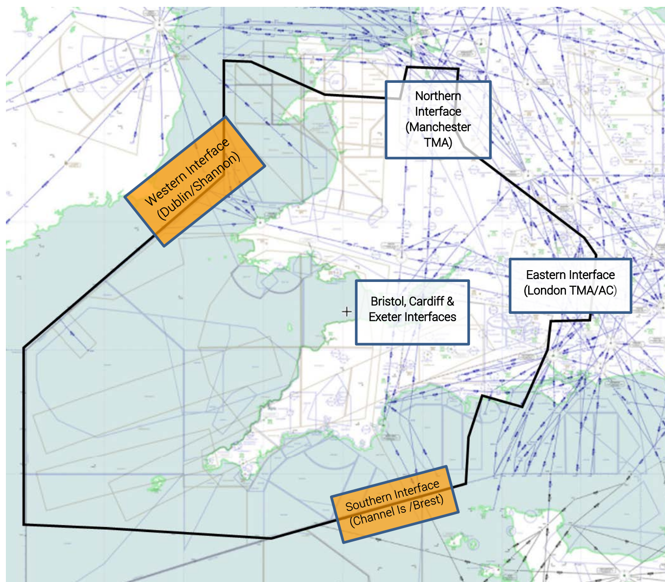
Figure 14: Location of interface options
