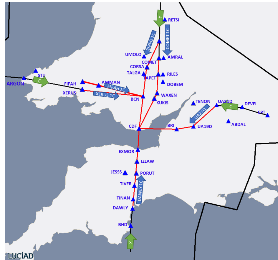
Figure 26 Cardiff proposed arrival connectivity
