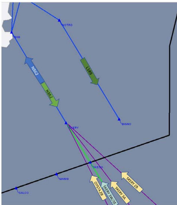
Figure 38 Channel Islands Group Extant Departure Connectivity
