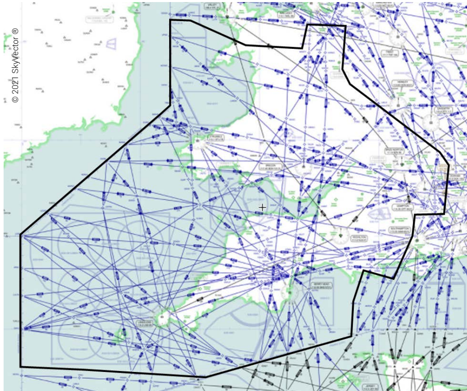
Figure 5: Upper ATS Routes (FL245 and above) within the LD1.1 area
