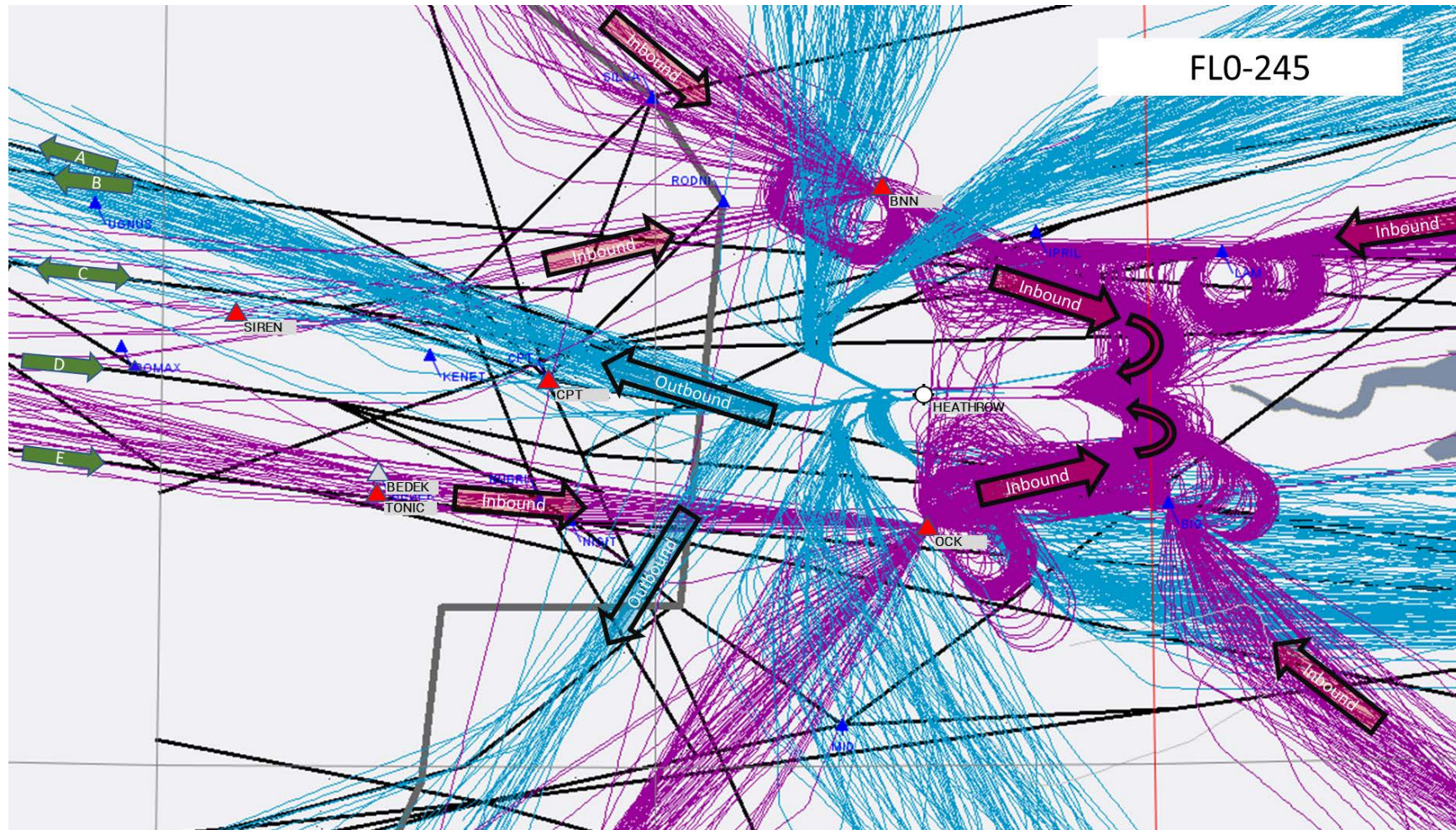
Figure 53 LTMA interface. Extant Heathrow Arrivals & Departures and proposed route structure (1 week – Aug 2019 data, below FL245, arrivals purple and departures blue) (note a separate pdf giving these trajectories layered by altitude is included in consultation materials. This allows you to assess the typical altitude of overflight in a particular location).
