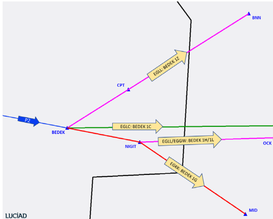
Figure 45 LTMA Extant arrival routes: BEDEK STARs (via P2)
