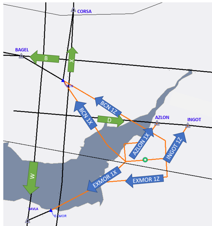
Figure 23 Bristol Proposed Departure Connectivity
