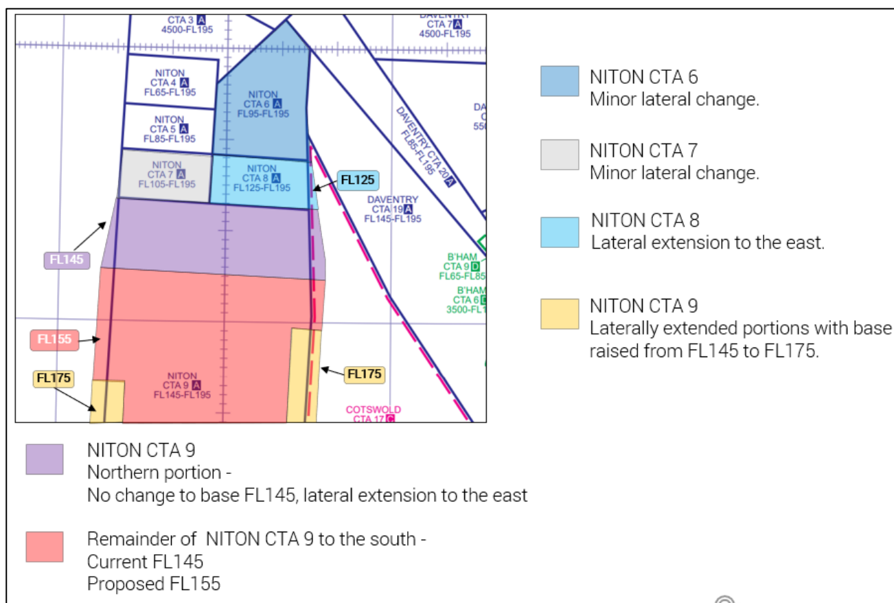
Figure 11 CAS changes: in NITON CTA
