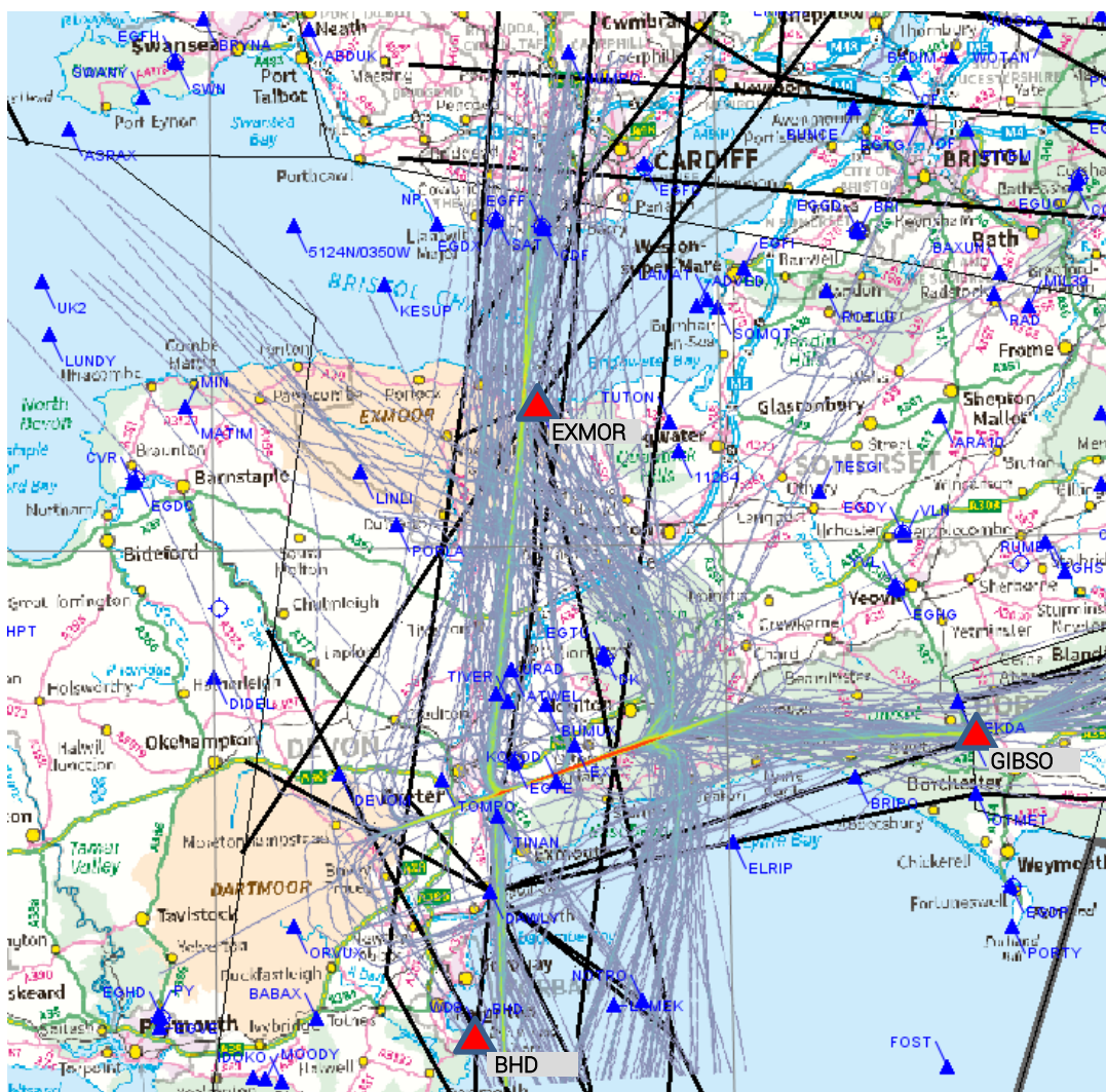
Figure 34 Exeter Extant flight paths shown over proposed route structure (1 week – Aug 2019 data, below FL245, arrivals and departures)
