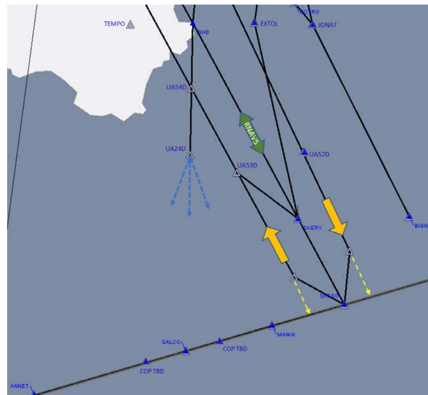
Figure 37 Brest Interface Connectivity (Option 6)
