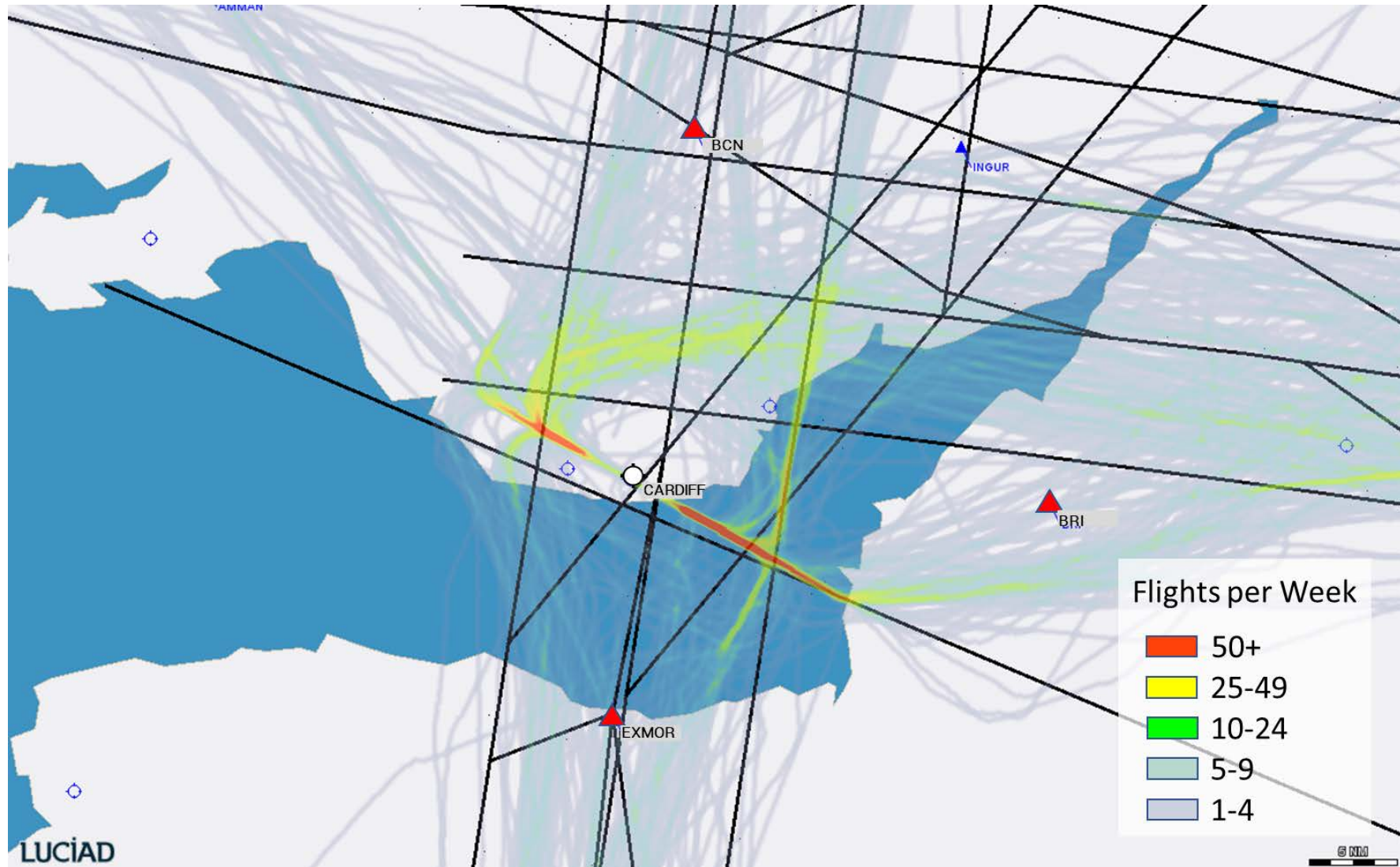
Figure 27 Cardiff, Extant flight paths shown over proposed route structure (1 week – Aug 2019 data, below FL245, arrivals and departures)
