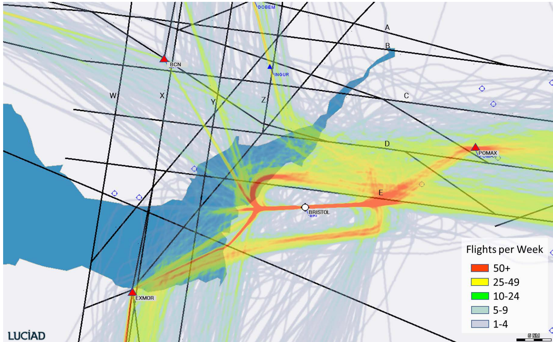
Figure 24 Bristol Current flight path pattern (1 week – Aug 2019 data, below FL245, arrivals and departures)
