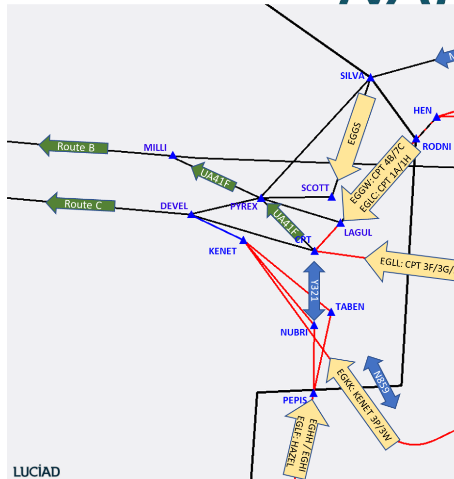
Figure 52 LTMA Proposed Departure connectivity via CPT
