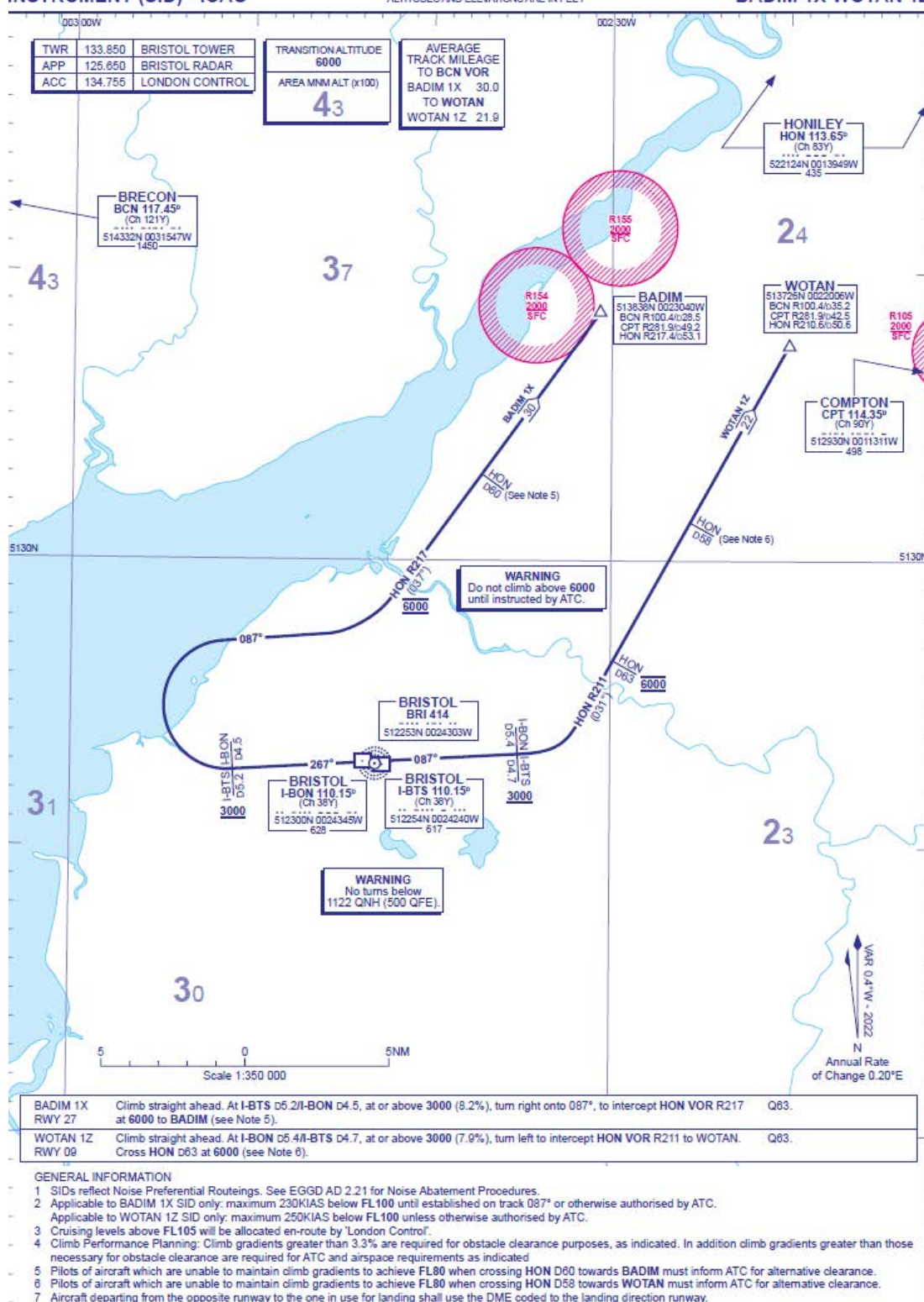
Figure 20 Extant Bristol BADIM 1X WOTAN 1Z SIDs
