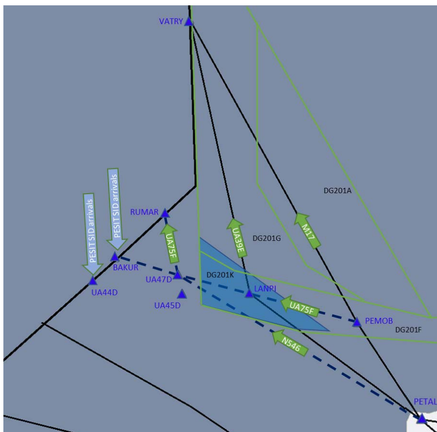
Figure 66 Option 6 Ireland Interface - proposed route structure
