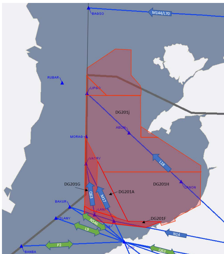
Figure 64 Extant Ireland Interface and D201
