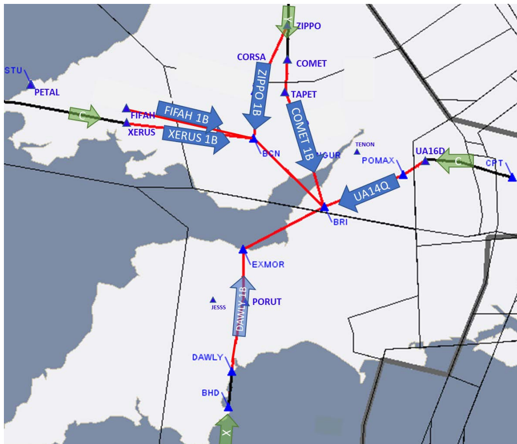
Figure 19 Bristol - Proposed Arrival Connectivity
