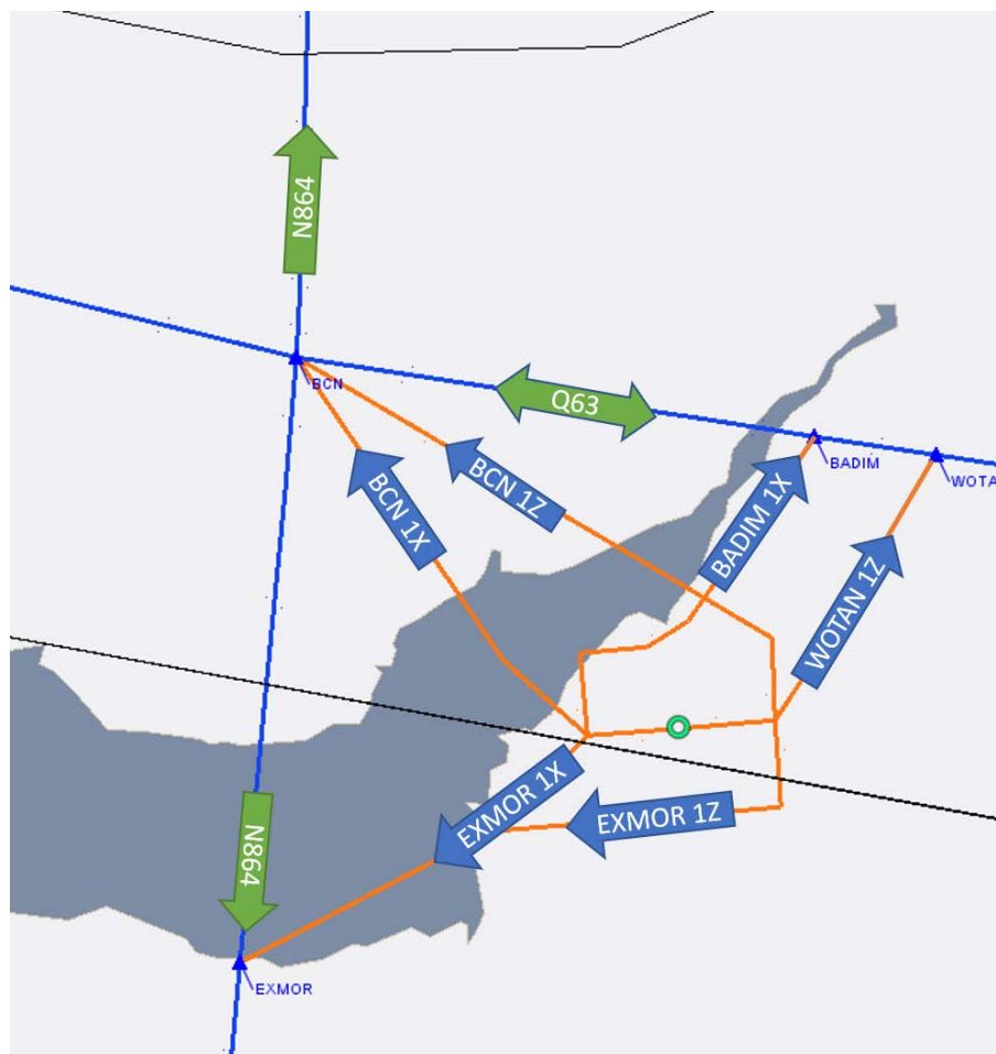
Figure 22 Bristol Baseline: Extant Departure Connectivity
