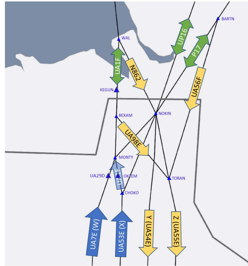
Figure 57 MTMA Proposed connectivity
