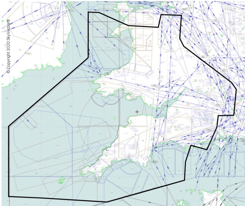
Figure 4: Lower ATS Routes (FL70 – 245) within the LD1.1 area
