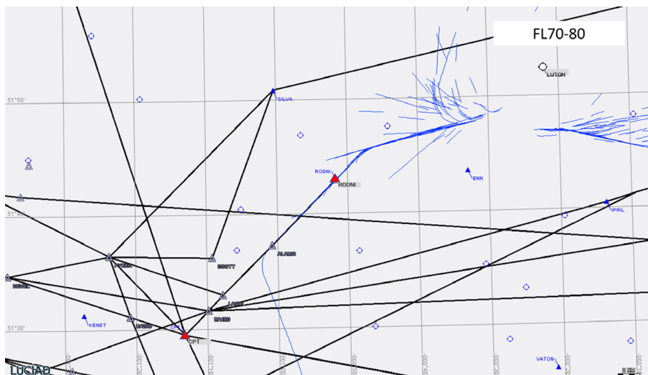
Figure 50 Luton departures on extant CPT 4B/7C SID (trajectories between FL70-80)
