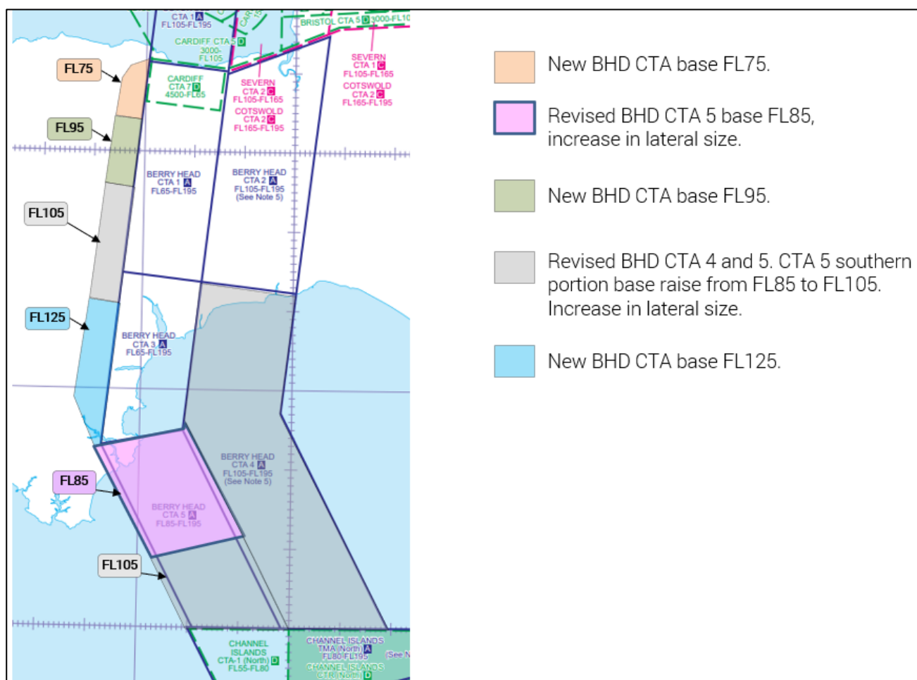
Figure 12 CAS changes: in BHD CTA
