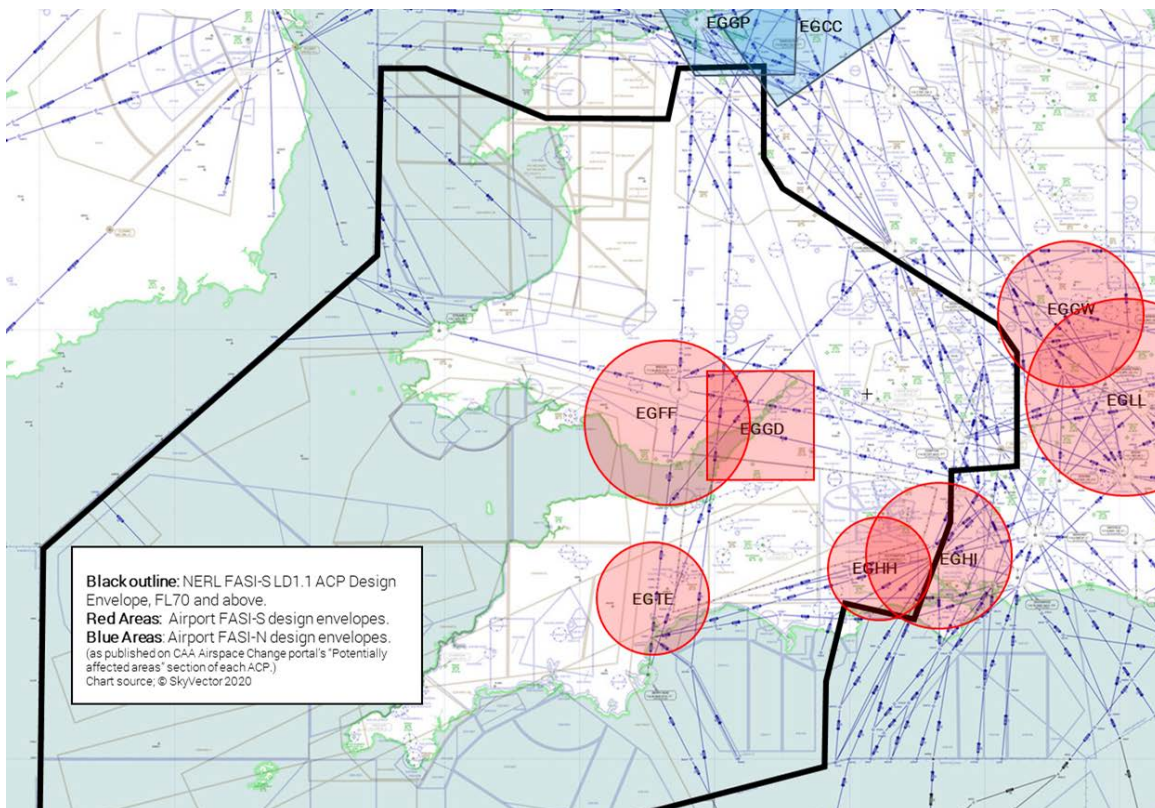
Figure 67 Other ACP interactions
