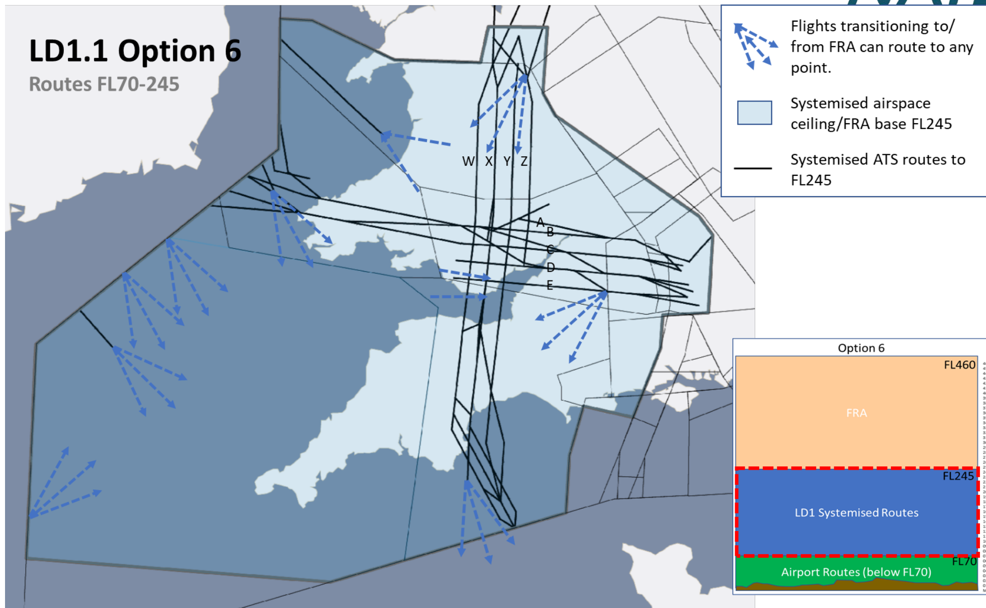
Figure 8 Option 6: Systemised routes FL70-245, with indicative FRA transitions from FL245
